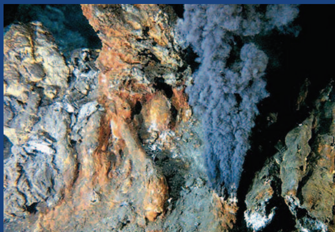
Black smoker (Photo courtesy of WHOI).
